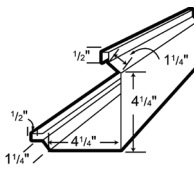
LG 123 "J" CHANNEL
